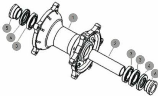
REAR HUBS
