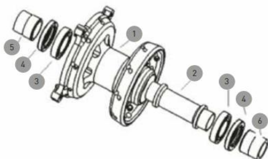
FRONT HUBS
